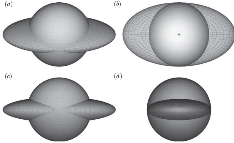
Figure 4. Deformation of a sphere of test particles in the case when one eigenvalue of -\Psi_{4ij}^{\text{nat}} is positive, one is zero and one is negative.
