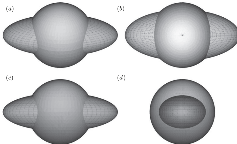
Figure 3. Deformation of a sphere of test particles in the case when one eigenvalue of -\Psi_{4ij}^{\text{nat}} is positive and two are negative.
