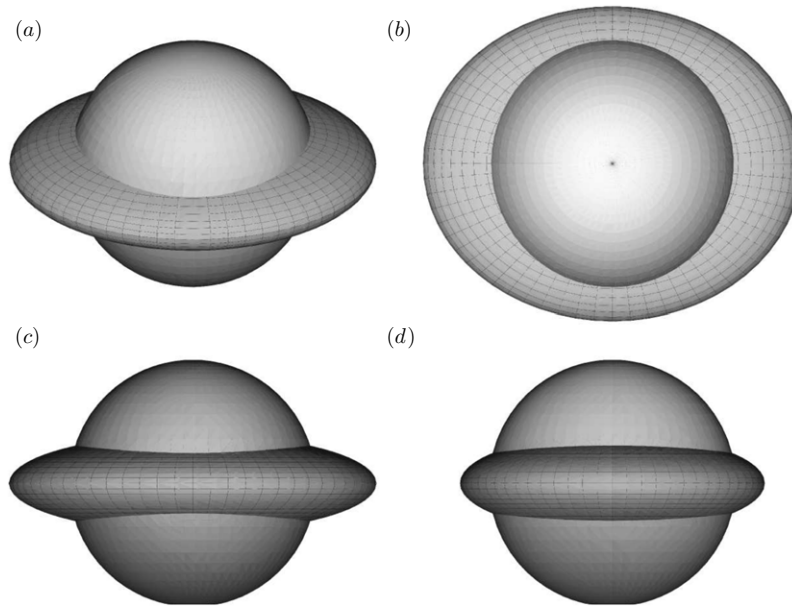
Figure 2. Deformation of a sphere of test particles in the case when two eigenvalues of -\Psi_{4ij}^{\text{nat}} are positive and one is negative ( D = 5 , the wave propagates in the direction e_{(1)} , and the transverse 3-space shown is spanned by e_{(2)}, e_{(3)}, e_{(4)} ). Plot (a) is a global view, (b), (c), (d) are views from the top, front, right, respectively.
