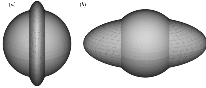
Figure 5. Deformation of a sphere of static test particles in the subtype D(b) when D = 5 for the cases (a) \Psi_{2S}^{\text{nat}} < 0 , (b) \Psi_{2S}^{\text{nat}} > 0 . Unlike in figures 2–4, here we show \mathbf{e}_{(1)}, \mathbf{e}_{(2)}, \mathbf{e}_{(3)} , where \mathbf{e}_{(1)} is the longitudinal direction (oriented horizontally) while \mathbf{e}_{(2)}, \mathbf{e}_{(3)} (plotted perpendicularly) are two directions of the transverse 3-space (the third equivalent transverse direction \mathbf{e}_{(4)} is suppressed).
