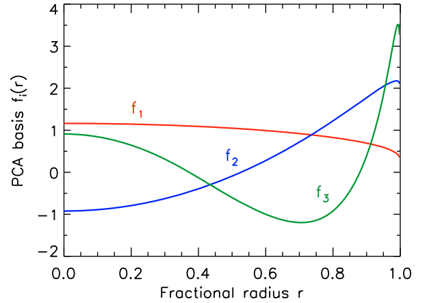
Fig. 5. First three basis functions of the PCA decomposition, computed for a set of atmosphere models that match the stellar parameters of OGLE 2004-BLG-482's source star.
