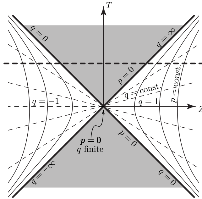
Figure 4. A section X = 0 (corresponding to t = 0 ) of the background Minkowski space for the Plebański–Demiański parameterisation with \epsilon_0 = 0 . The surfaces on which p > 0 is a constant are rotational hyperboloids -T^2 + X^2 + Z^2 = p^2 around the expanding/contracting cylinder X^2 + Z^2 = T^2 , arbitrary Y = y , on which p = 0 , q = \pm\infty . The surfaces on which q is constant are planes through the spacelike line on which T = 0 = Z , with X, Y arbitrary. The horizontal heavy dashed line indicates the section T = \text{const.} through the space-time that is illustrated in figure 5. The shaded regions are not covered by the Plebański–Demiański coordinates.
