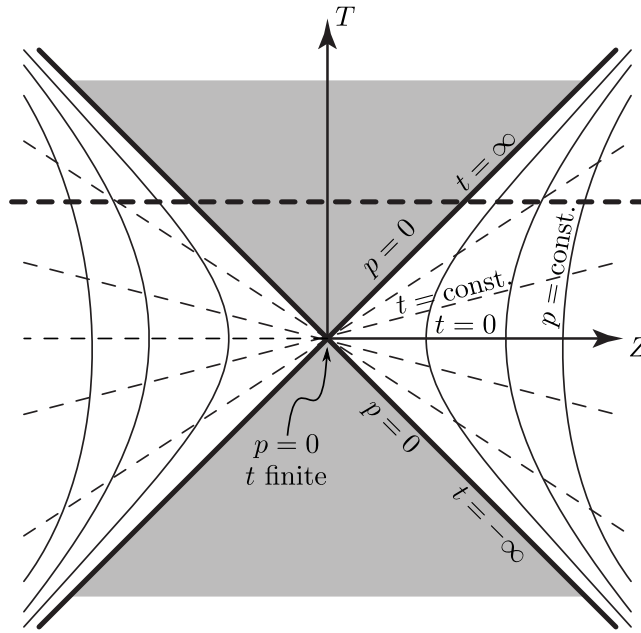
Figure 2. A section of the background flat space on which X = 0 (corresponding to q = 0 ) and Y = y is any constant. For all three Plebański–Demiański coordinate parameterisations of Minkowski space with \epsilon_0 = +1, 0, -1 , the surfaces on which p > 0 is a constant are rotational hyperboloids -T^2 + X^2 + Z^2 = p^2 around the expanding (for T > 0 ) or contracting (for T < 0 ) cylinder X^2 + Z^2 = T^2 , Y arbitrary. The coordinate singularity p = 0 is located along the Y -axis ( T = 0 , X = 0 = Z , Y arbitrary). The surfaces on which t is constant are planes through the spacelike line on which T = 0 = Z , with X, Y arbitrary. The horizontal heavy dashed line indicates the section T = \text{const.} through the space-time that is illustrated in figure 3. The shaded regions are not covered by the Plebański–Demiański coordinates.
