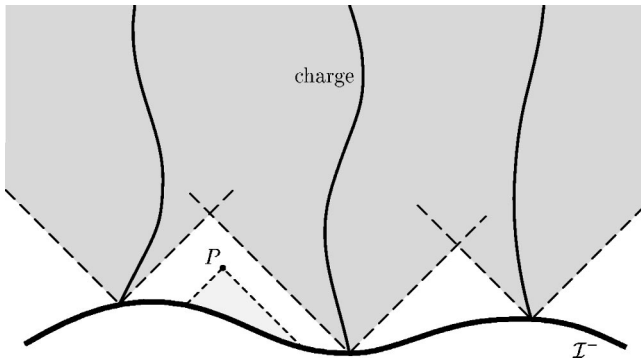
FIG. 1. Fields at spacelike \mathcal{I}^- . When past infinity \mathcal{I}^- is spacelike, and some discrete sources “enter” the spacetime, then incoming fields must necessarily be present at \mathcal{I}^- and also at such points as P , the past null cones of which are not crossed by the worldlines of the sources. If this is not the case, inconsistencies arise. The past null cone of P is shaded in light gray, whereas the future domain of influence of sources is shaded in dark gray. (Figure taken after Penrose [9].)
