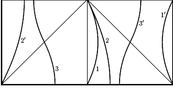
FIG. 4. Worldlines of particles in de Sitter spacetime. The worldlines of geodesics and of uniformly accelerated particles in de Sitter spacetime, obtained by the conformal transformation of appropriate worldlines in Minkowski space: 1,1' from the worldline of a particle moving uniformly through the origin, 2,2' from a particle at rest outside the origin, and 3,3' from two uniformly accelerated particles. In de Sitter space, the worldlines 1 and 1' describe two uniformly accelerated particles; 2,2' and 3,3' are geodesics. Both particles in each pair are causally disconnected.
