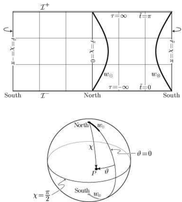
Figure 2: The spherical cosmological coordinates and a pair of uniformly accelerated particles w_{\ominus} and w_{\oplus} in de Sitter universe: the conformal diagram (above) and projection on the spacelike cut \tau = \text{constant} in the standard cosmological spherical coordinates (angle \varphi suppressed). The whole de Sitter spacetime could be represented by just the “right half” of the conformal diagram. For convenience, we admit negative values of radial coordinates and identify \tilde{r} = \chi = -\pi and \tilde{r} = \chi = \pi (see the text below Eq. (3.12) and the Appendix).
