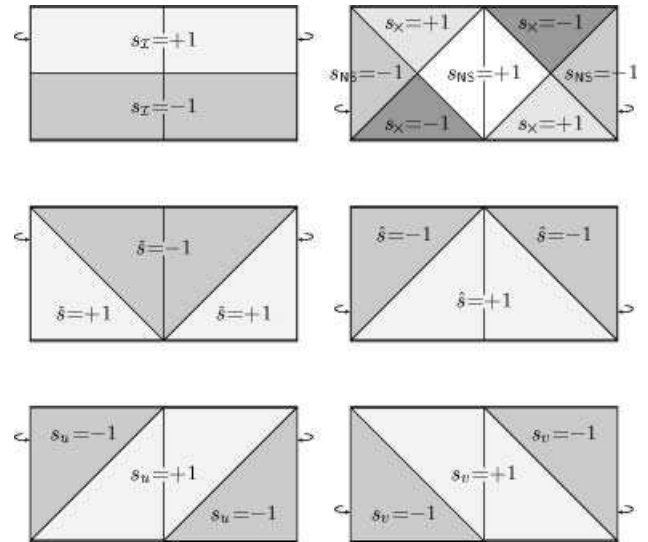
Figure 13: The values of the factors s_T , s_{NS} , s_X , \hat{s} , \hat{s} , s_u and s_v in various regions of de Sitter space. The factors are defined in Eqs. (A73), (A61), (A74), (A21), (A36) and (A128), respectively. The factor s_X is used only in the expressions for static coordinates in the region where the Killing vector is spacelike. Therefore, we indicated the values of s_X only in those regions, although Eq. (A74) defines s_X everywhere. The factors s_X , s_u , and s_v are defined only for any given section \vartheta = \text{constant} , but not as unique functions on the whole spacetime (they are not symmetric with respect to the pole). This is related to our convention using negative radial coordinates, cf. the text below Eq. (A1).
