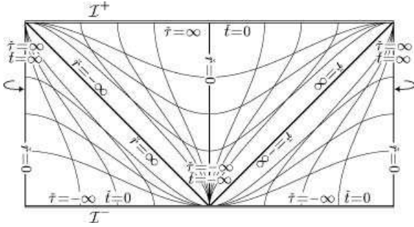
Figure 15: The flat cosmological family, type “ \vee ”.
