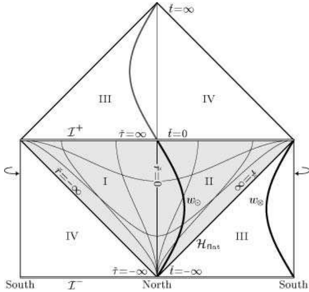
Figure 3: The flat cosmological coordinates and particles w_{\odot} , w_{\infty} in de Sitter space and in conformally related Minkowski space. The flat cosmological coordinates cover shaded region. Its boundary, \tilde{r} = \pm\infty , represents the horizon for observers at rest in these coordinates.
