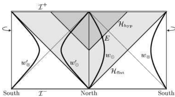
Figure 7: The worldlines of uniformly accelerated charges. The particles w_\ominus and w'_\ominus start and end at the “north pole,” w_\otimes , w'_\otimes start and end at the south pole. Particles w'_\otimes , w'_\ominus have a higher magnitude of acceleration a_{\text{ds}} than particles w_\otimes , w_\ominus . They are characterized by a negative parameter \alpha_o , whereas particles w_\otimes , w_\ominus have a positive \alpha_o .
