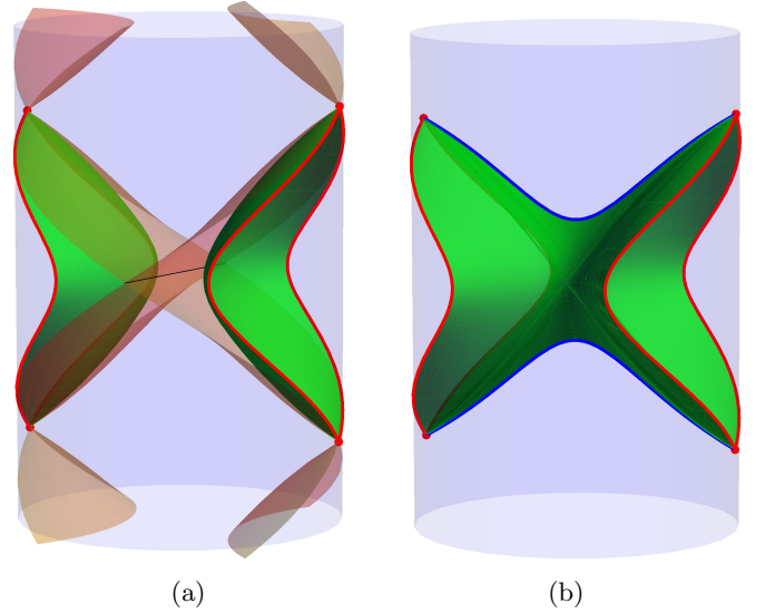
Figure 3. World-sheets of minimal surfaces. Vertical cylinder represents 3+1 dimensional AdS spacetime with angular direction \varphi suppressed. The world-sheet of one circular boundary is thus reduced only to two curves at infinity. One circular boundary is localized in the left static region, other in the right one. (a) Two uniformly accelerated hyperplanes spanned on these circular boundaries. Killing horizons are indicated. (b) The world-sheet of the tube-like minimal surface joining the same circular boundaries.
