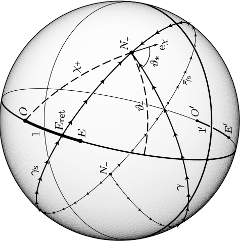
Figure 5. Space trajectories of null geodesics \gamma , \gamma_s and \bar{\gamma}_s indicated on the slice \tilde{t} = \text{constant} ( \varphi = 0 ). Charges 1, 1' move along \vartheta = 0 from poles O , O' to points E , E' and back. \gamma , \gamma_s and \bar{\gamma}_s start at N_- at \tilde{t} = 0 and arrive at N_+ (with coordinates \chi_+ , \vartheta_+ ) at \tilde{t} = \pi . The direction of \gamma at N_+ is specified by angles \vartheta_* , \varphi_* ( \varphi_* describes rotation around e_x in the dimension not seen). \gamma_s crosses the worldline of particle 1 at E_{\text{ret}} , \bar{\gamma}_s reaches N_+ from the opposite direction.
