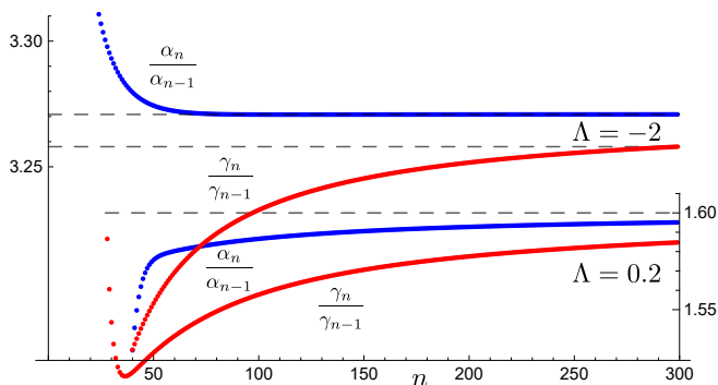
FIG. 1. The convergence radius can be estimated from the ratio convergence test for solutions (4.4), (4.5), here given by r_h = -1 , k = 0.5 with b = 0.3 , \Lambda = 0.2 (bottom) and b = 0.2 , \Lambda = -2 (top).
