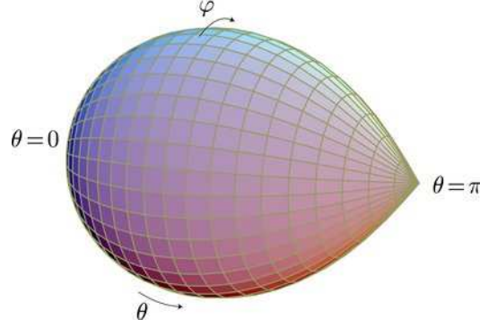
Figure 3: The surface of constant t and r illustrated as an embedding into E^3 . This is regular at \theta = 0 , but there is a conical singularity at \theta = \pi corresponding to the deficit angle \delta_\pi = \frac{8\pi\alpha m}{1+2\alpha m} .
