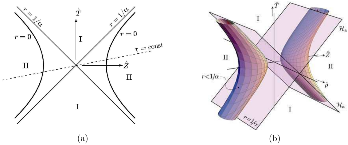
Figure 4: In the weak field limit of the C -metric, a causally separated pair of test particles at r = 0 accelerate away from each other in opposite spatial directions as illustrated in (a). The acceleration horizon at r = 1/\alpha is given by \hat{Z} = \pm \hat{T} . For r < 1/\alpha , surfaces r = \text{const.} enwrap the accelerated particles at r = 0 as depicted in (b).
